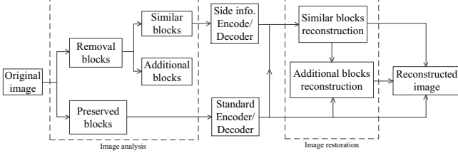
Fig. 1. The flowchat of proposed image compression scheme.
