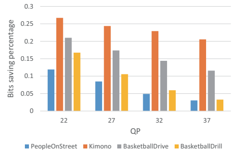
Fig. 4. Raw bits saving for different QP.
